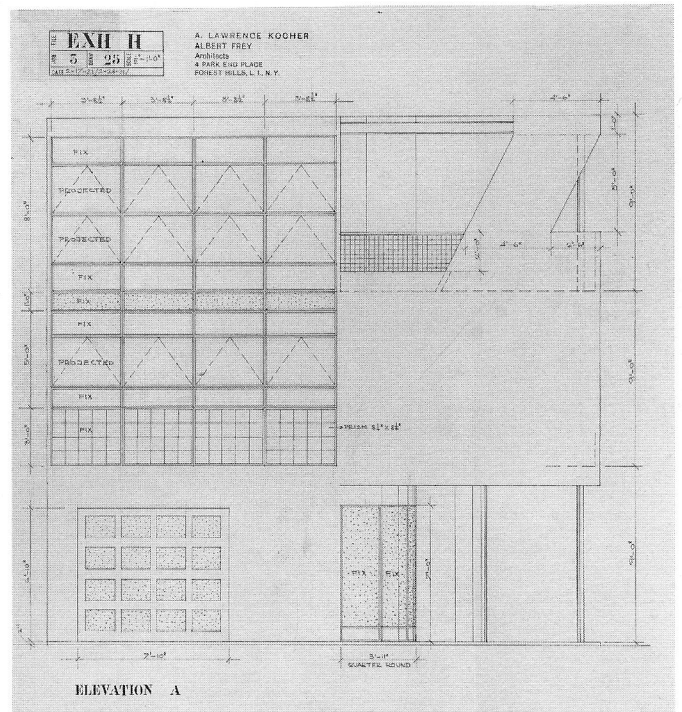
23. Drawing of west elevation
