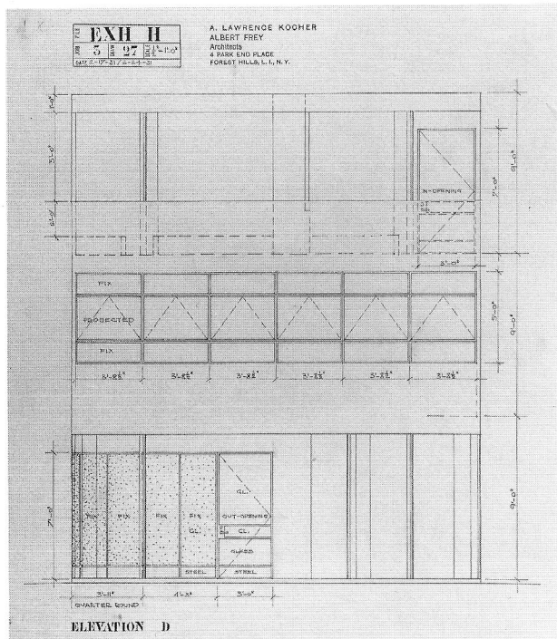
21. Drawing of south elevation
